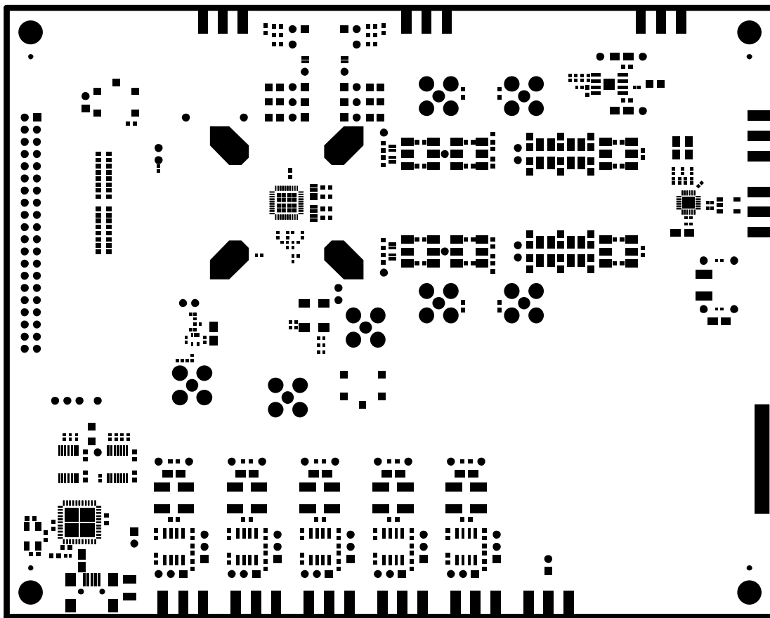
Figure 133. Solder Mask—Primary Side, No Socket
