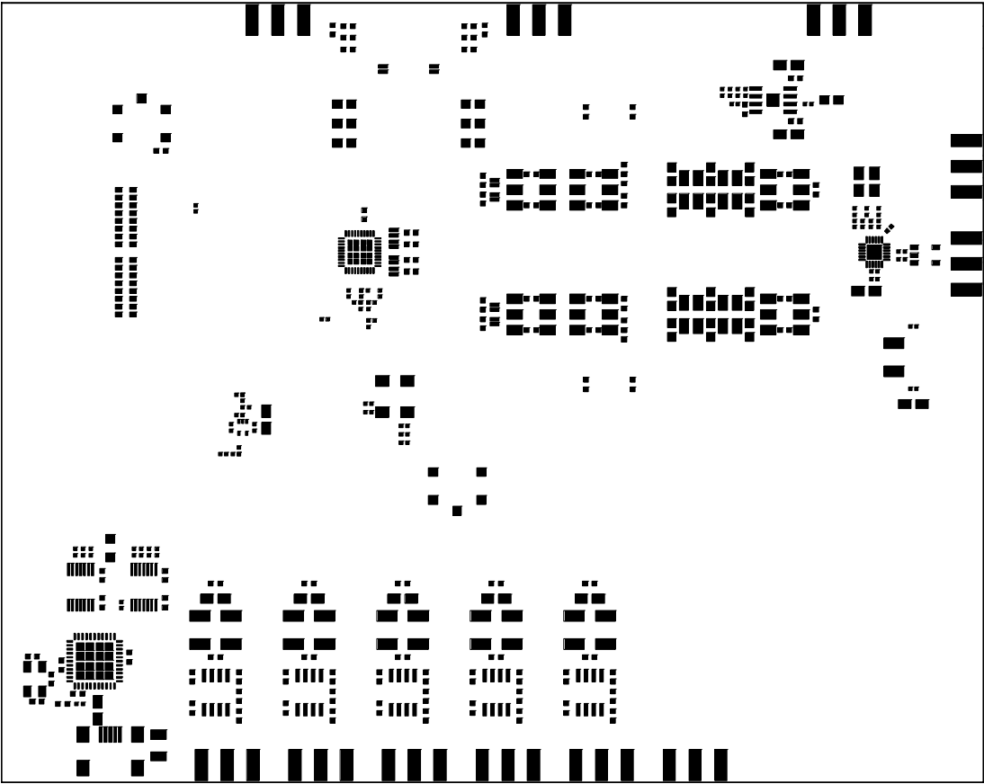
Figure 126. Primary Side Paste
