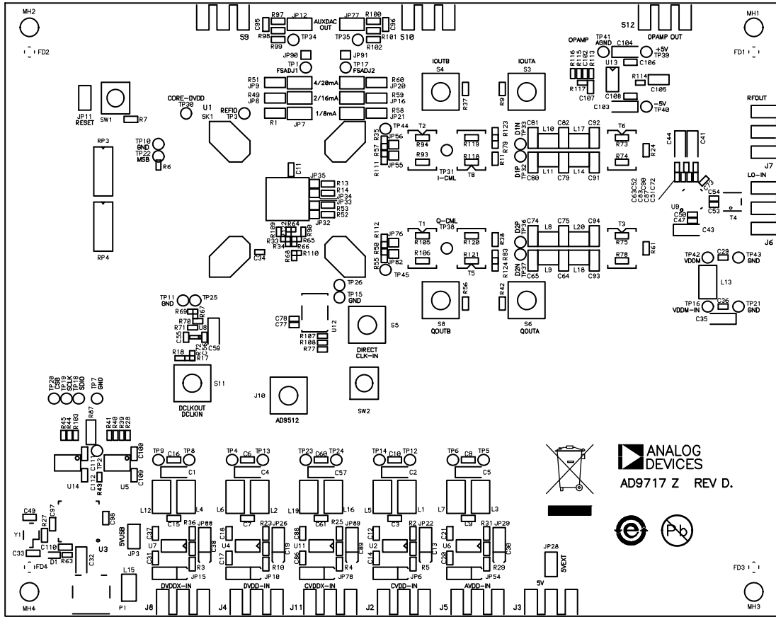
Figure 128. Silkscreen—Primary Side
