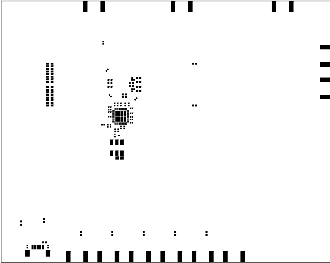
Figure 127. Secondary Side Paste
