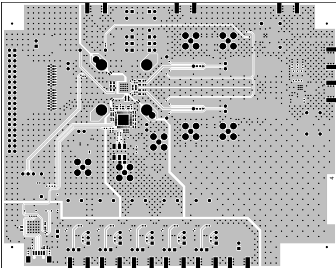
Figure 131. Layer 4—Secondary Side
