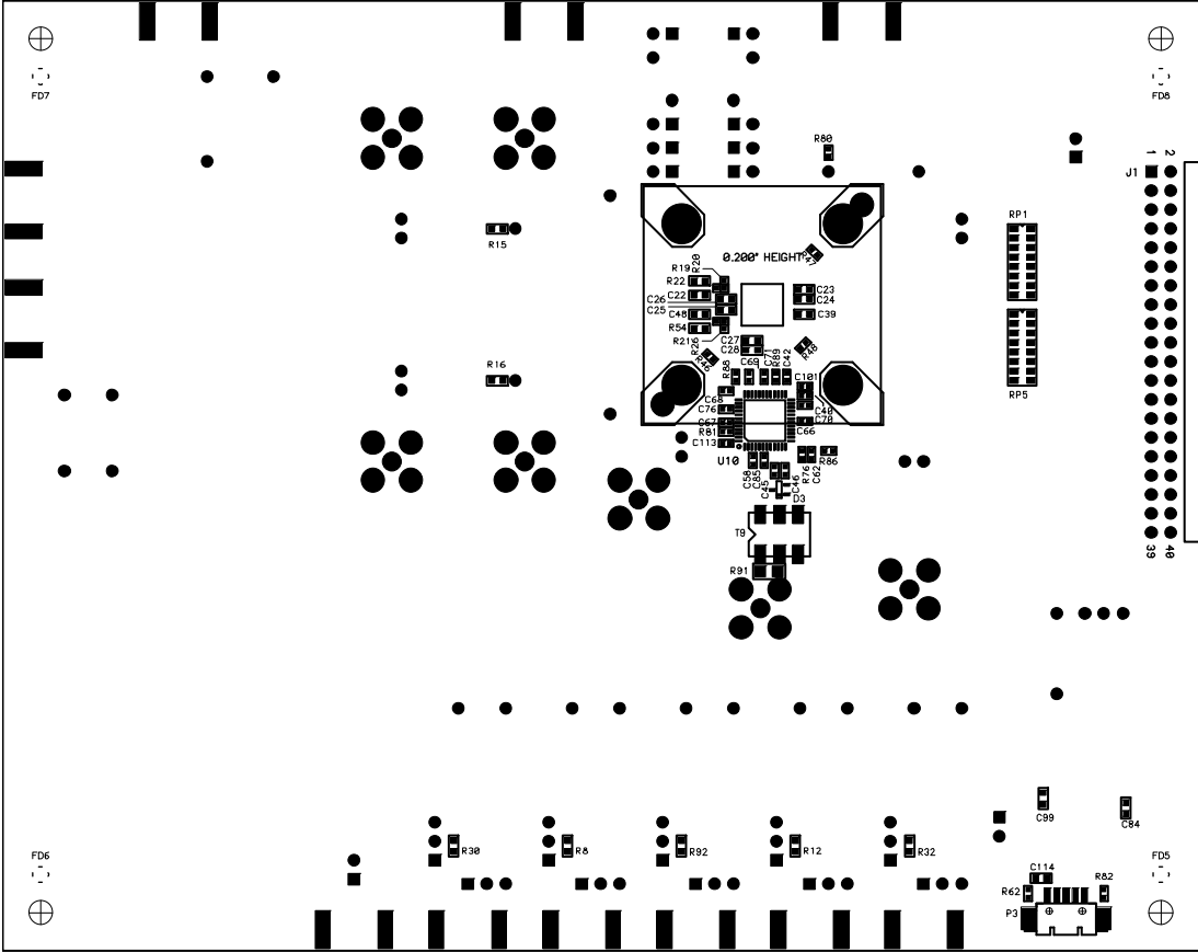
Figure 122. Assembly—Secondary Side
