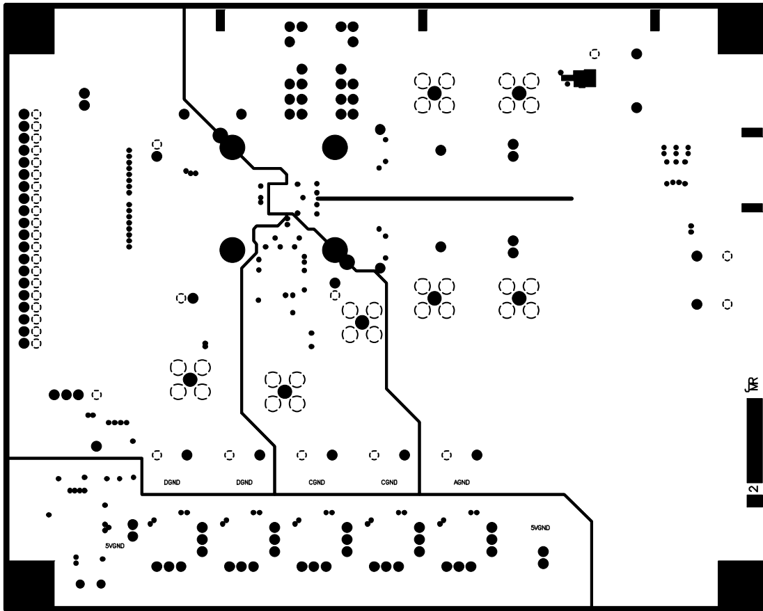
Figure 119. Layer 2, Ground Plane
