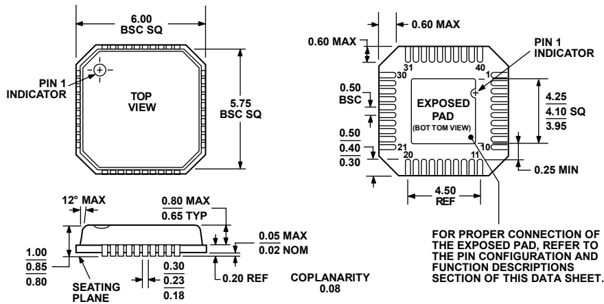
Figure 134. 40-Lead Lead Frame Chip Scale Package [LFCSP_VQ] 6 mm × 6 mm, Very Thin Quad (CP-40-1) Dimensions shown in millimeters
