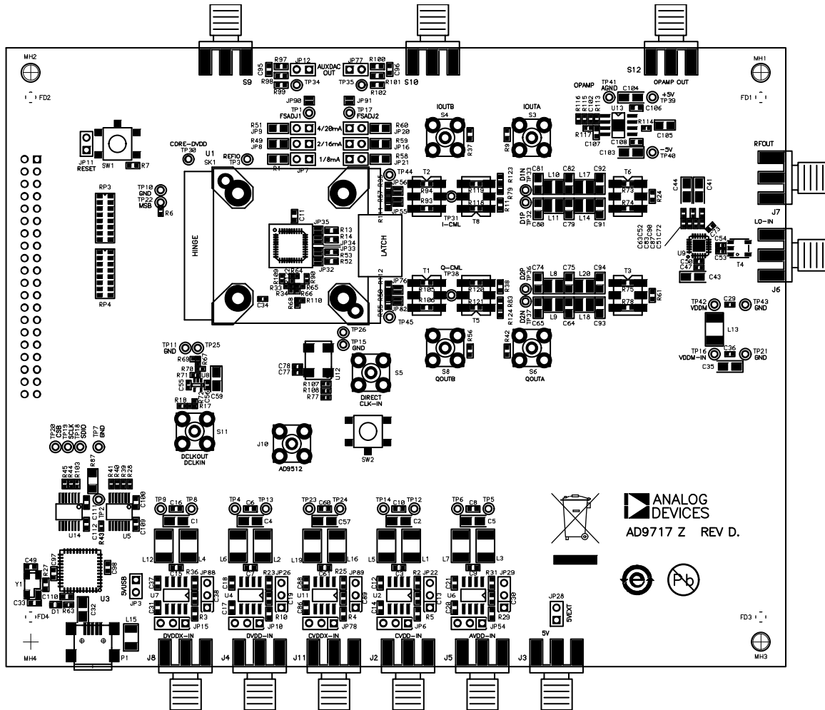
Figure 121. Assembly—Primary Side
