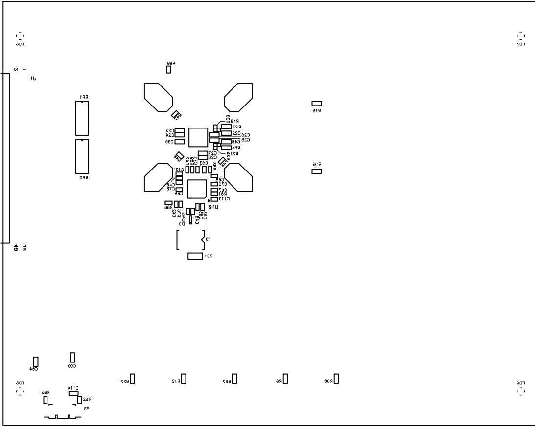
Figure 129. Silkscreen—Secondary Side
